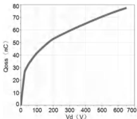
Figure 7. Typical Qoss
