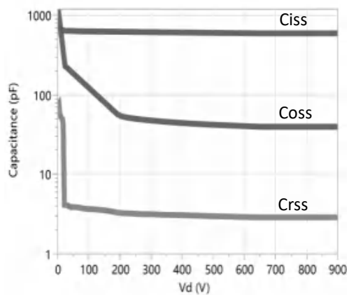
Figure 5. Typical Capacitance
