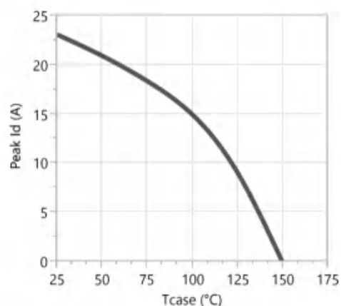
Figure 9. Current Derating
