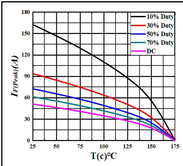
Figure 3. Current Derating
