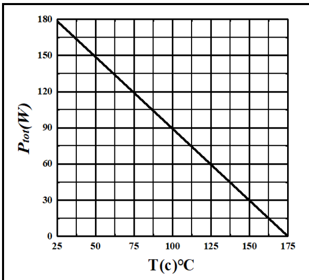
Figure 5. Power Derating
