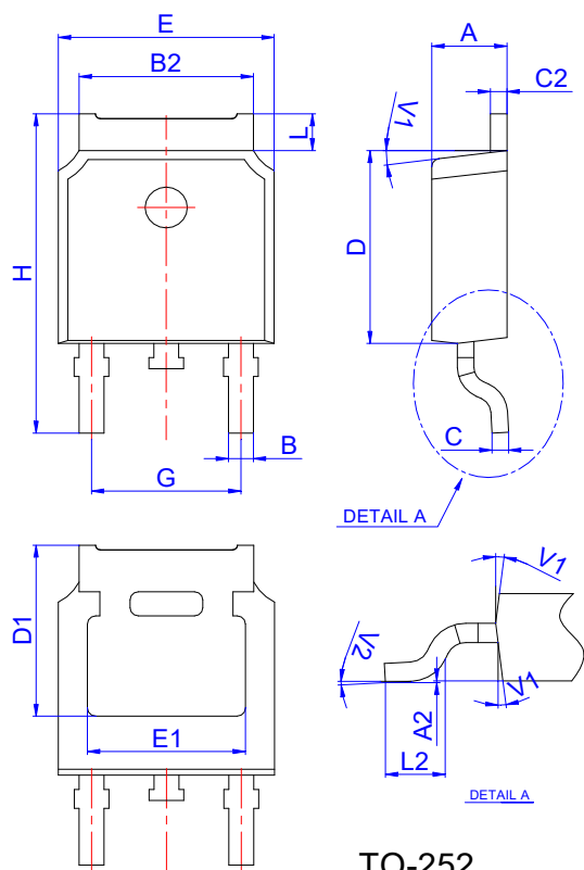
TO-252
