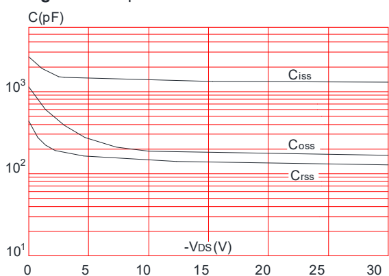
Figure 6: Capacitance Characteristics
