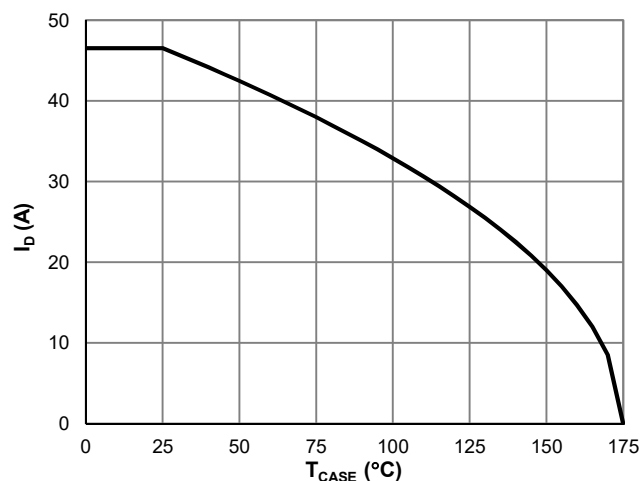
Figure 7: Current De-rating
