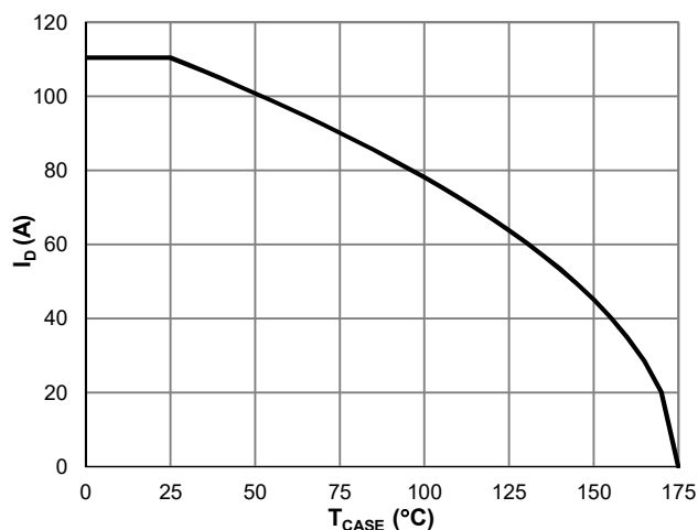
Figure 7: Current De-rating
