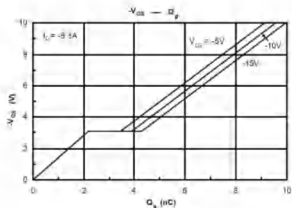
电参数曲线图 / Electrical Characteristic Curve
