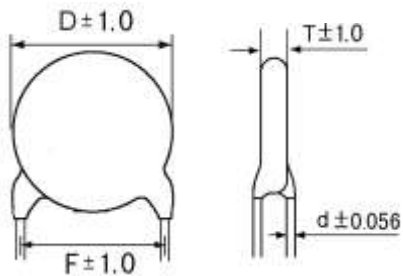
成品尺寸 (Product Dimensions)
